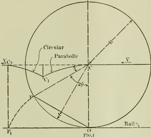
C 1 C 2 is path of centre of wheel from when C 2 O is vertical until C P is vertical
